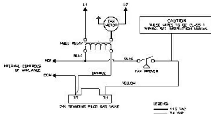
HST CONNECTED TO 24V STANDING PILOT
