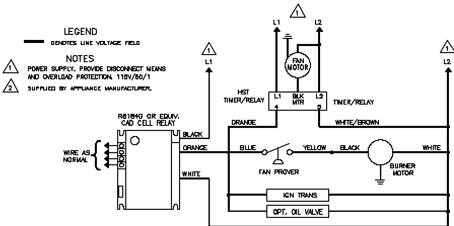
HST CONNECTED TO AN R8184G BURNER MOTOR LESS THAN 3 AMPS @ 120 VAC
