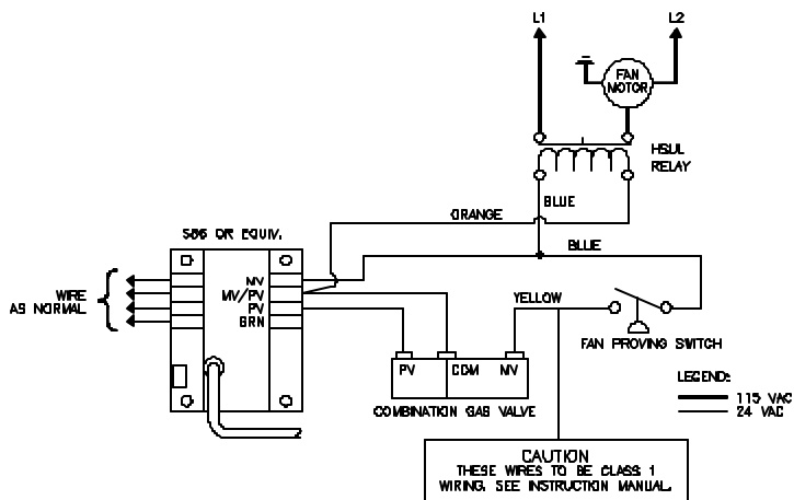
HSUL CONNECTED TO 24V ELECTRONIC IGNITION
